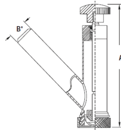
VO3 SERIES OPERATORS STAINLESS STEEL DIMENSIONS
