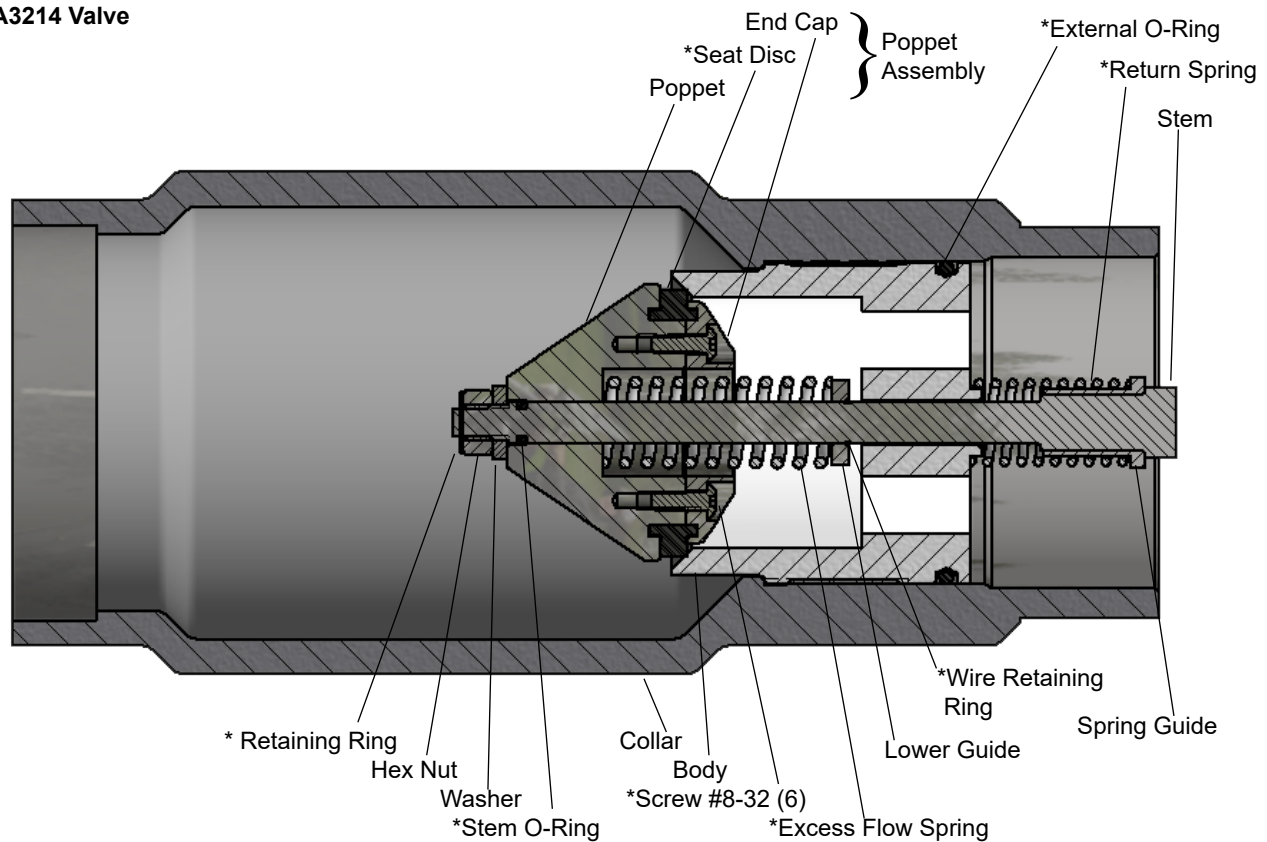
Figure 2 - A3214 Valve
