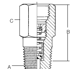
SS8021, SS8022 Series (.156" Orifice)***
