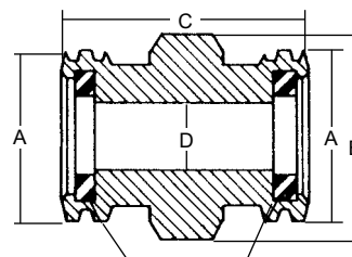
Gasket (Furnished with adapter) ACME x ACME
