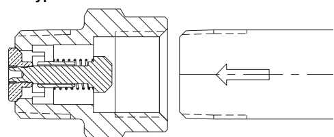
Typical Installation
