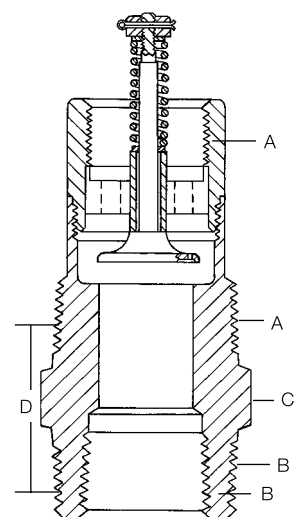
Typical Installations
