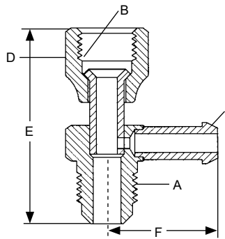
Female Inverted Flare x Male NPT
