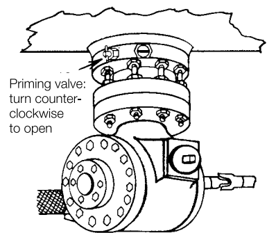
Figure 6. Priming Procedures
